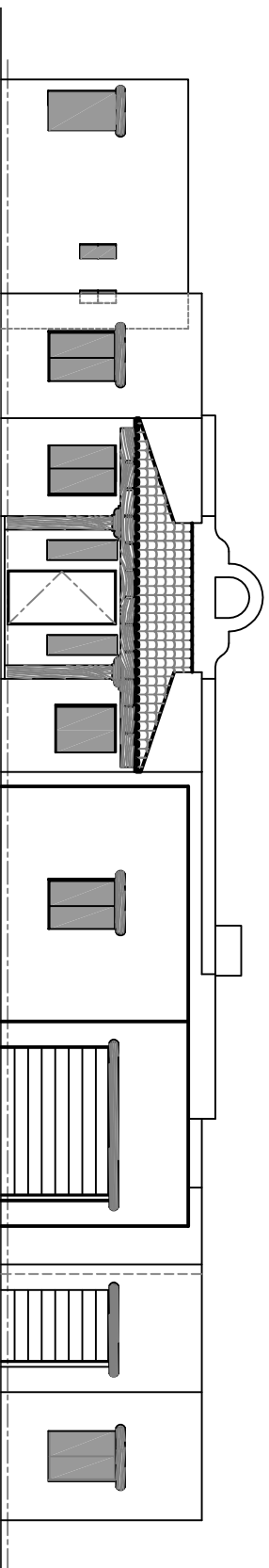
Front Elevation - "A"
